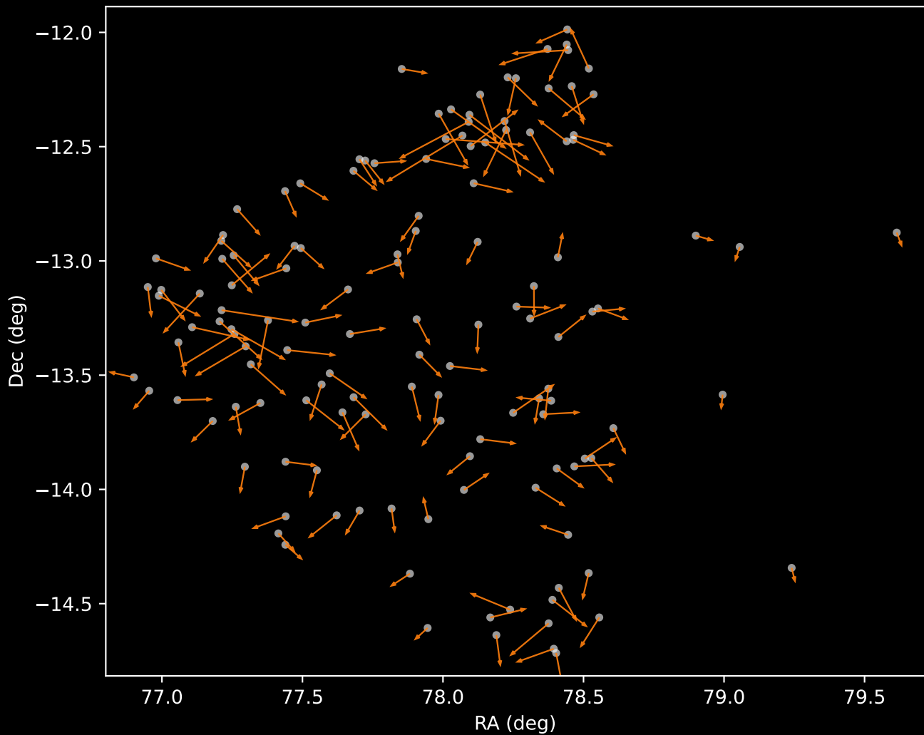
APOGEE DR17 Cluster 2 Proper Motion Vectors (n=134)
