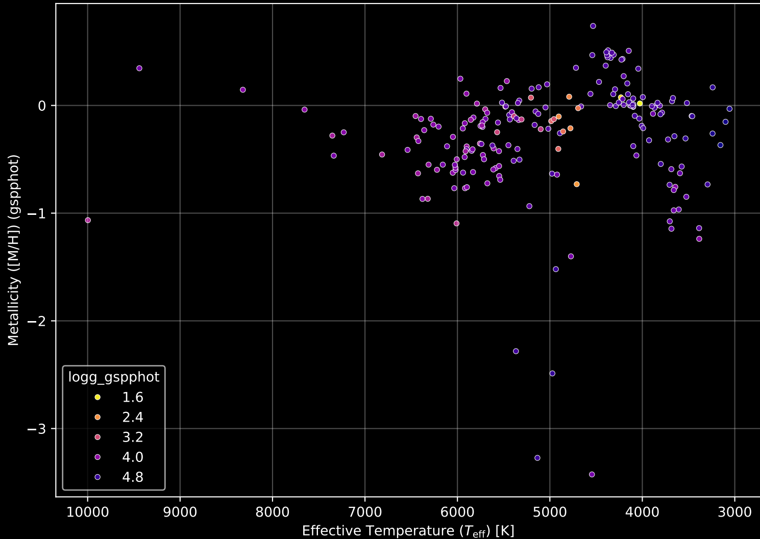
APOGEE DR17 Field: [K2_C3_049-55] Stellar Population Parameters (n= 201)
