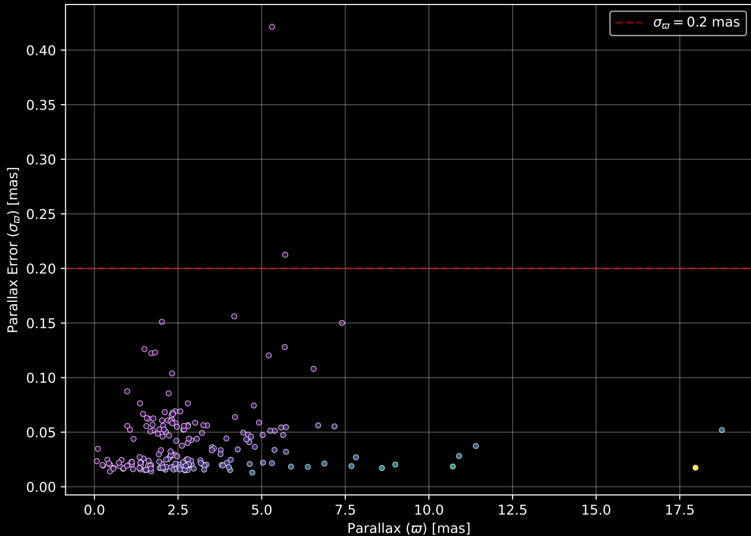
APOGEE DR17 Field: [K2_C3_049-55] Parallax Quality (n= 201)
