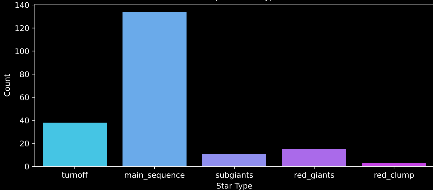
APOGEE DR17 Field: [K2_C3_049-55] Count plot of Star Type
