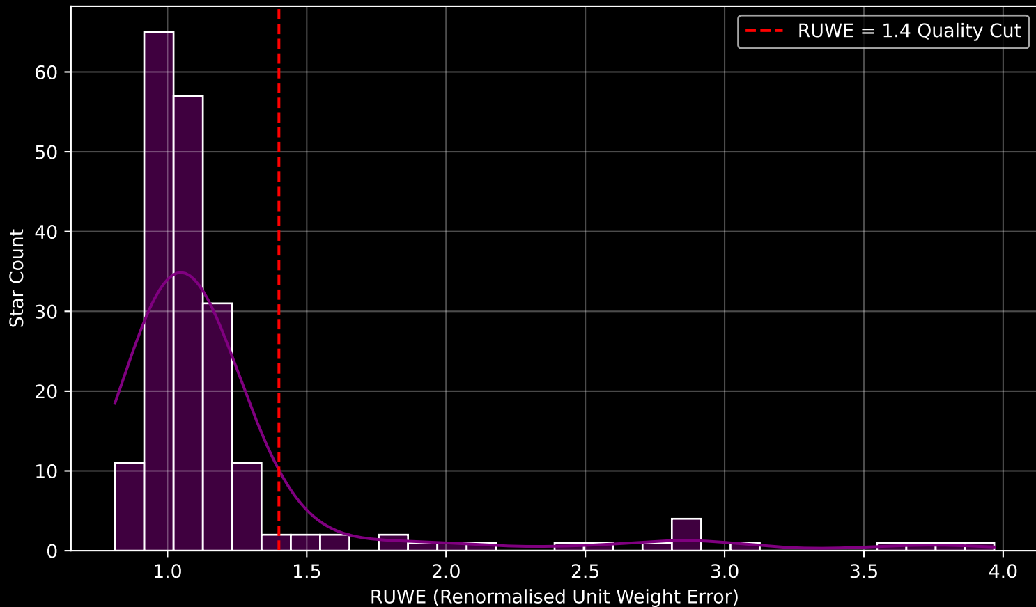
GAPOGEE DR17 Field [K2_C3_049-55] RUWE Distribution (n= 198)
