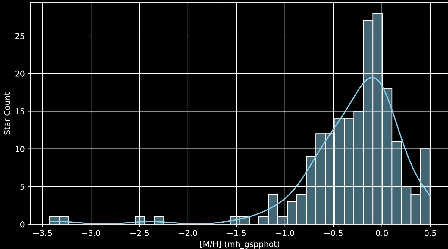
APOGEE DR17 Field: [K2_C3_049-55 [M/H] (mh_gspphot) (n= 198)
