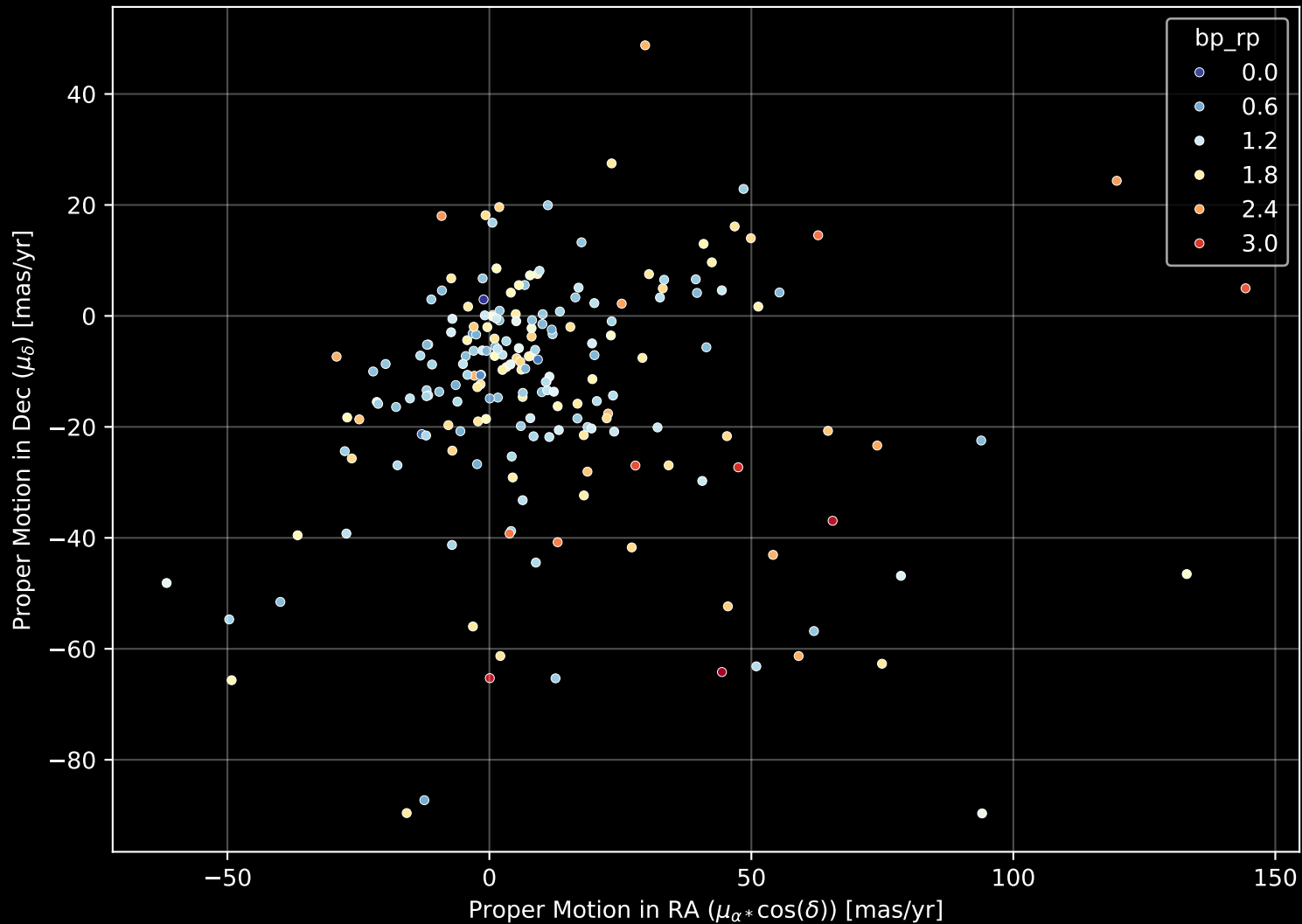
APOGEE DR17 Field: [K2_C3_049-55] Proper Motion Diagram (n= 201)
